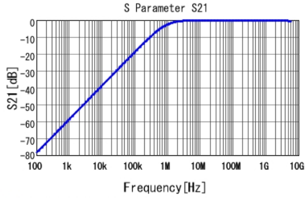
■ GCD188R71H182KA01 S21 DCOV, 25degC
