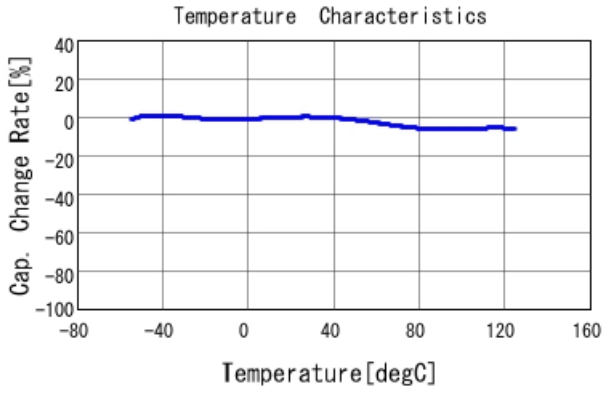
■ GCD188R71H182KA01 C-Temp. capchange, DCO. 0V, AC1. 0V rm
