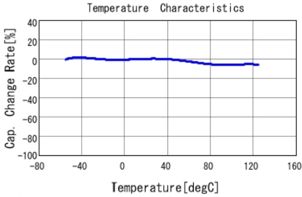
■ GCD188R71H272KA01 C-Temp. capchange, DCO. 0V, AC1. 0Vrm
