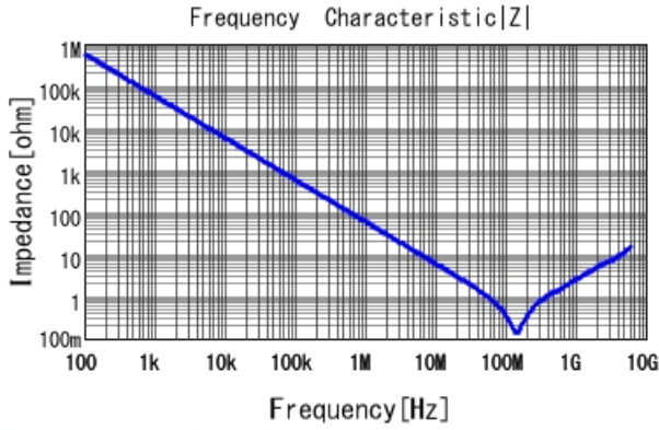
GCD188R71H272KA01 |Z| DC0V, 25degC
