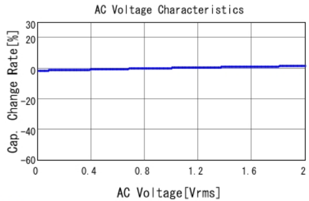
GCD188R71H272KA01 C-AC Voltage capchange, DC0V, 25.0d
