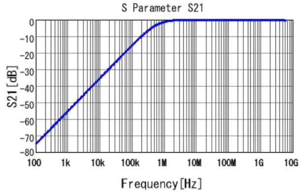
■ GCD188R71H272KA01 S21 DCOV, 25degC
