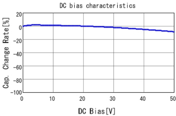
GCD188R71H272KA01 C-DC bias capchange, 25.0degC, AC1.
