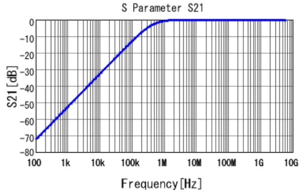
■ GCD188R71H392KA01 S21 DCOV, 25degC
