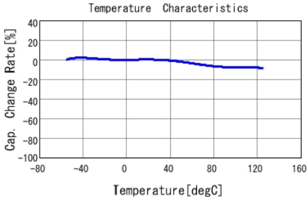
■ GCD188R71H392KA01 C-Temp. capchange, DCO. 0V, AC1. 0Vrm
