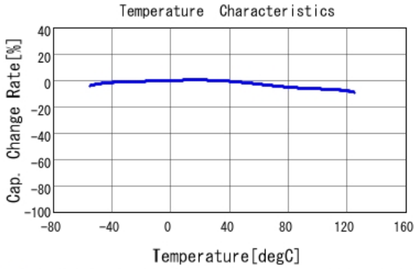
■ GCD188R71H562KA01 C-Temp. capchange, DCO. 0V, AC1. 0V rm
