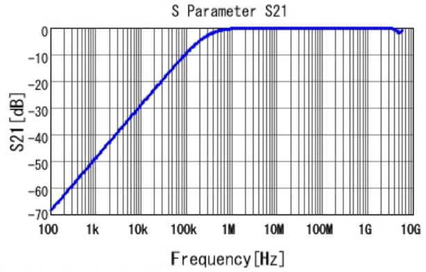
■ GCD188R71H562KA01 S21 DCOV, 25degC
