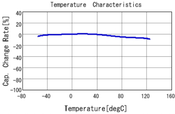
■ GCD188R72A562KA01 C-Temp. capchange, DCO. 0V, AC1. 0Vrm
