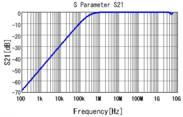
■ GCD188R72A562KA01 S21 DCOV, 25degC
