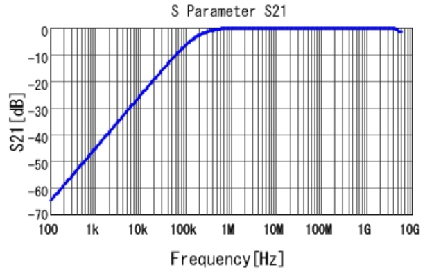
■ GCD188R72A822KA01 S21 DCOV, 25degC
