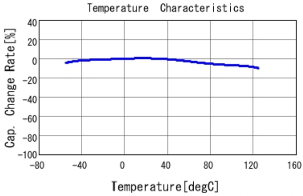
■ GCD188R72A822KA01 C-Temp. capchange, DCO. 0V, AC1. 0Vrm
