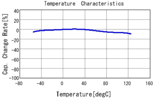
■ GCD21BR71H393KA01 C-Temp. capchange, DCO. 0V, AC1. 0Vrm
