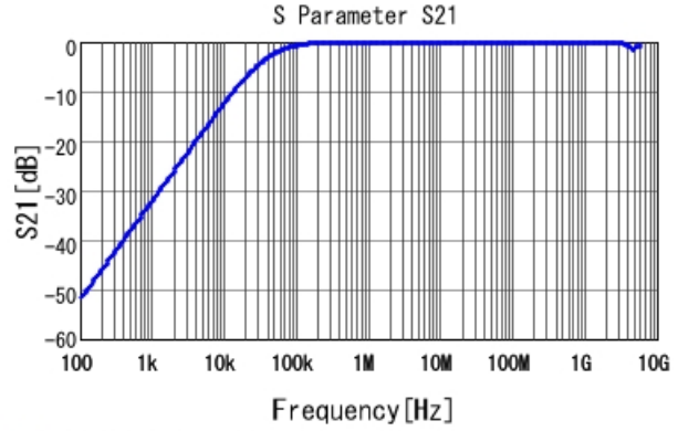
■ GCD21BR71H393KA01 S21 DCOV, 25degC
