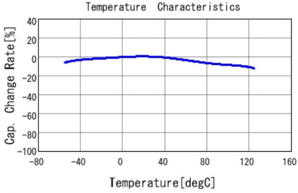
■ GCD21BR71H563KA01 C-Temp. capchange, DCO. 0V, AC1. 0Vrm
