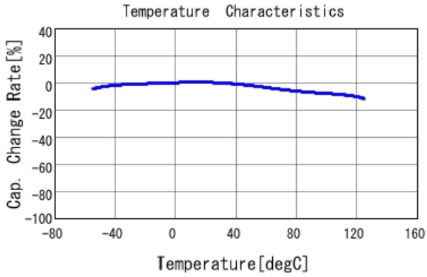
GCD21BR72A104KA01 C-Temp. capchange, DCO. 0V, AC1. 0Vrm
