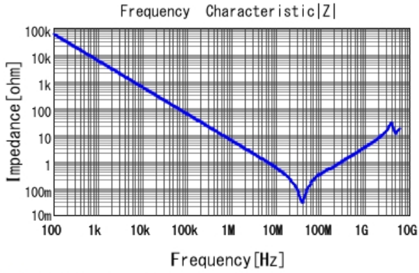
■ GCD21BR72A273KA01 |Z| DC0V, 25degC
