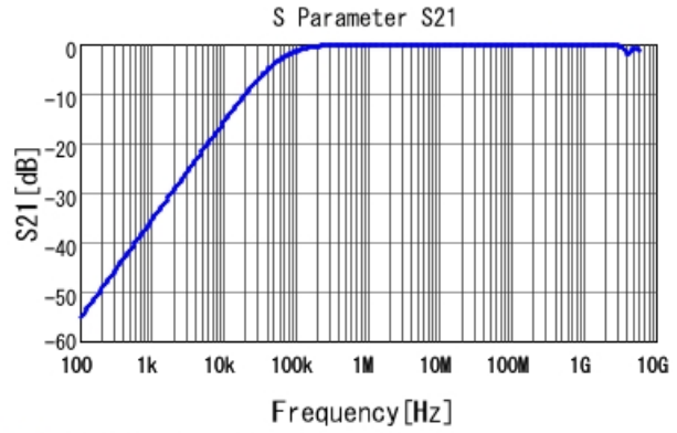
■ GCD21BR72A273KA01 S21 DCOV, 25degC
