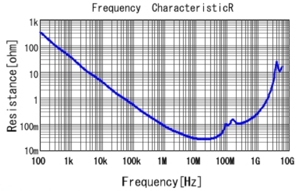
■ GCD21BR72A273KA01 R DC0V, 25degC
