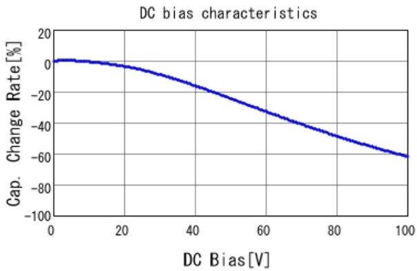
■ GCD21BR72A273KA01 C-DC bias capchange, 25.0degC, AC1.
