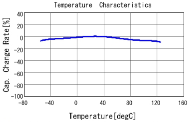
■ GCD21BR72A273KA01 C-Temp. capchange, DCO. 0V, AC1. 0Vrm
