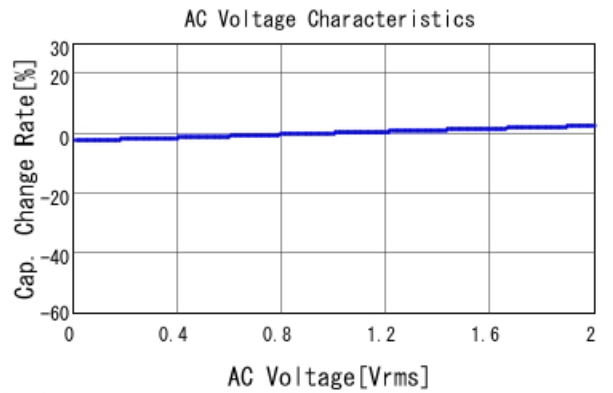
■ GCD21BR72A273KA01 C-AC Voltage capchange, DC0V, 25.0d
