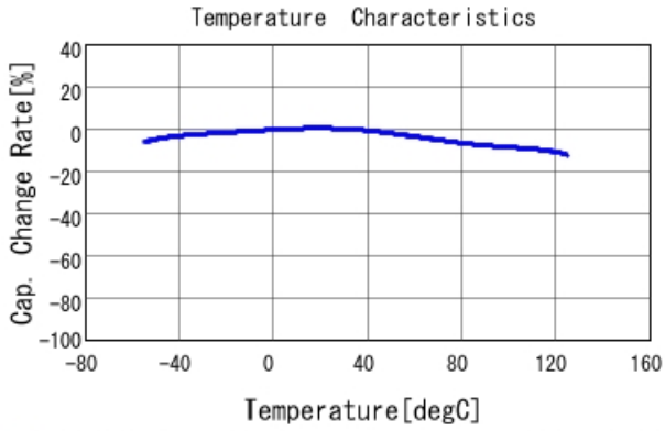
■ GCD21BR72A563KA01 C-Temp. capchange, DCO. 0V, AC1. 0Vrm
