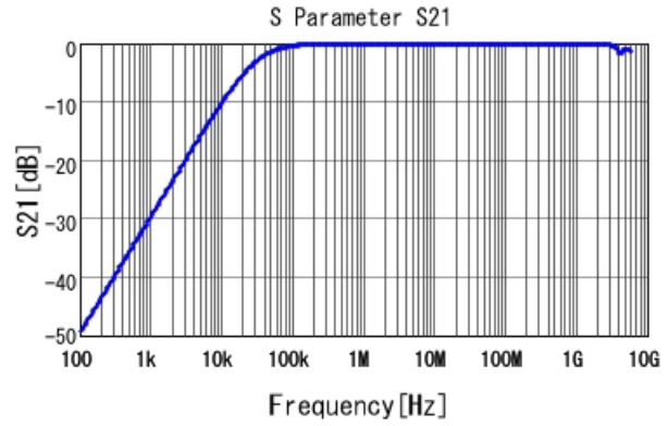
■ GCD21BR72A563KA01 S21 DCOV, 25degC
