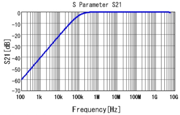
■ GCE188R72A153KA01 S21 DCOV, 25degC
