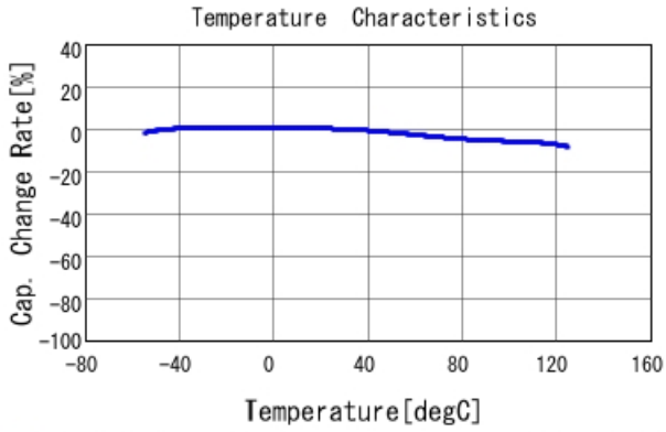
■ GCE188R72A153KA01 C-Temp. capchange, DCO. 0V, AC1. 0Vrm
