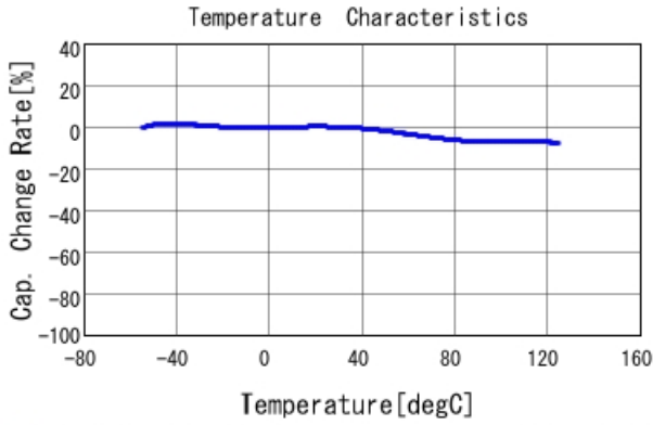
■ GCE188R72A392KA01 C-Temp. capchange, DCO. 0V, AC1. 0Vrm
