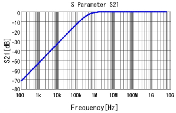
■ GCE188R72A392KA01 S21 DCOV, 25degC
