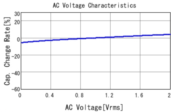
■ GCJ188L81E224KA01 C-AC Voltage capchange, DC0V, 25.0d
