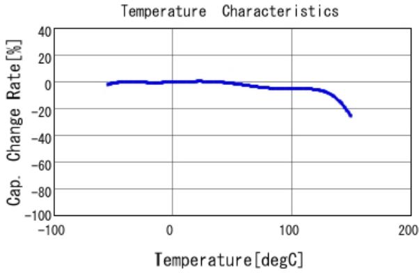
■ GCJ188L8YA333KA01 C-Temp. capchange, DCO. 0V, AC1. 0Vrm
