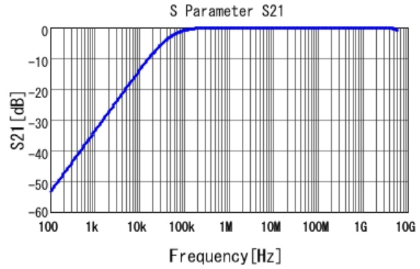
■ GCJ188L8YA333KA01 S21 DCOV, 25degC
