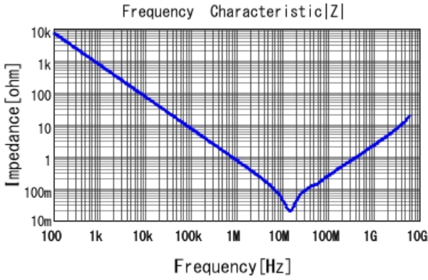
■ GCJ188R71A224KA01 |Z| DC0V, 25degC
