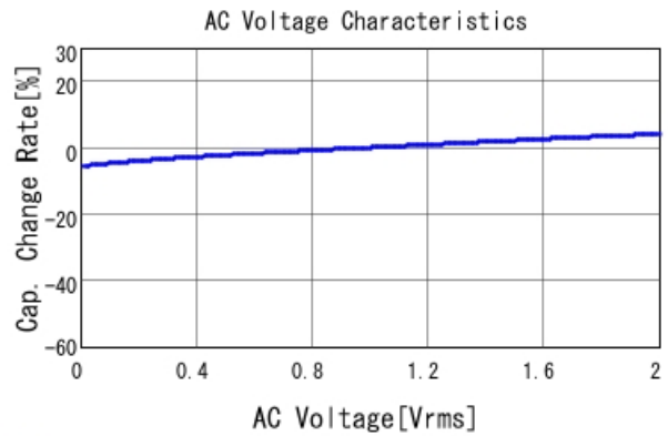
■ GCJ188R71A224KA01 C-AC Voltage capchange, DC0V, 25.0d
