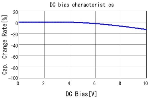
■ GCJ188R71A224KA01 C-DC bias capchange, 25.0degC, AC1.
