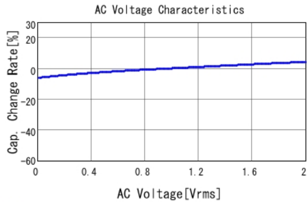
■ GCJ188R71C274KA01 C-AC Voltage capchange, DC0V, 25.0d
