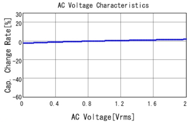
■ GCJ188R71E153KA01 C-AC Voltage capchange, DC0V, 25.0d
