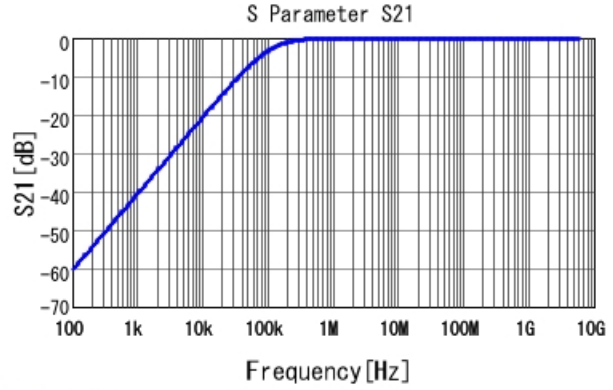
■ GCJ188R71E153KA01 S21 DCOV, 25degC
