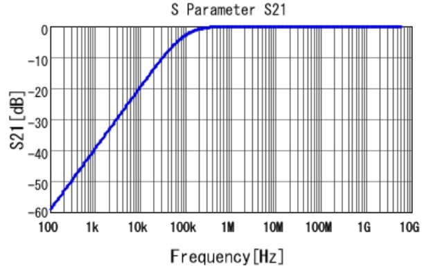
■ GCJ188R71E183KA01 S21 DCOV, 25degC
