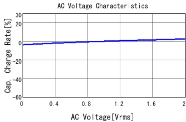
■ GCJ188R71E183KA01 C-AC Voltage capchange, DC0V, 25.0d
