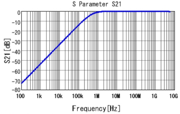
■ GCJ188R71E332KA01 S21 DCOV, 25degC
