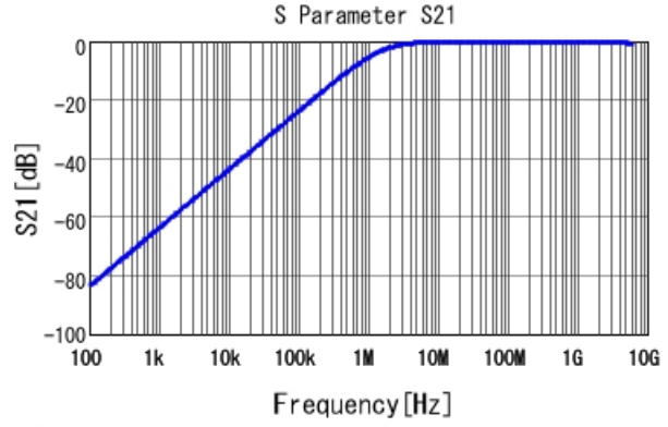
■ GCJ188R71H102KA01 S21 DCOV, 25degC
