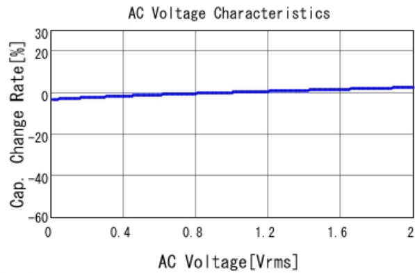
■ GCJ188R71H224KA01 C-AC Voltage capchange, DC0V, 25.0d
