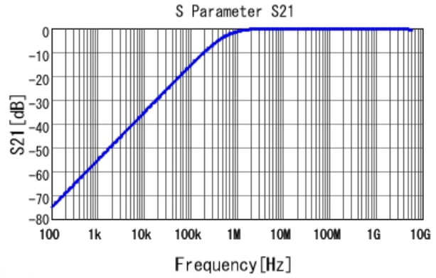
■ GCJ188R71H272KA01 S21 DCOV, 25degC
