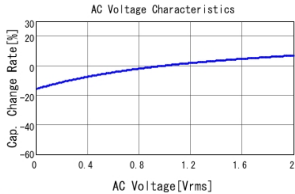
■ GCJ188R91E474KA01 C-AC Voltage capchange, DC0V, 25.0d
