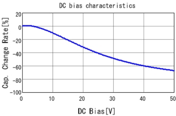
■ GCJ188R91H154KA01 C-DC bias capchange, 25.0degC, AC1.
