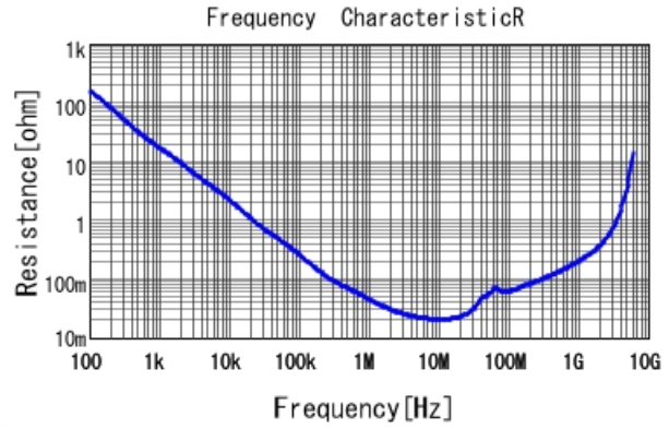
■ GCJ188R91H154KA01 R DCOV, 25degC
