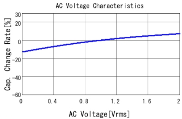
■ GCJ188R91H154KA01 C-AC Voltage capchange, DCOV, 25.0d
