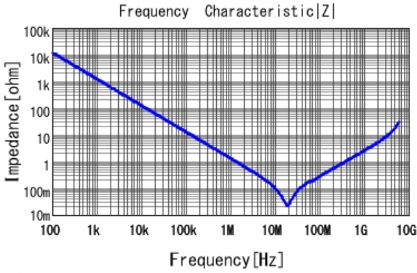
■ GCJ188R91H154KA01 |Z| DCOV, 25degC
