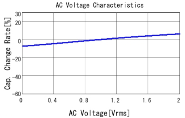
■ GCJ188R92A223KA01 C-AC Voltage capchange, DC0V, 25.0d
