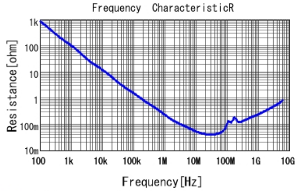
■ GCJ188R92A223KA01 R DC0V, 25degC
