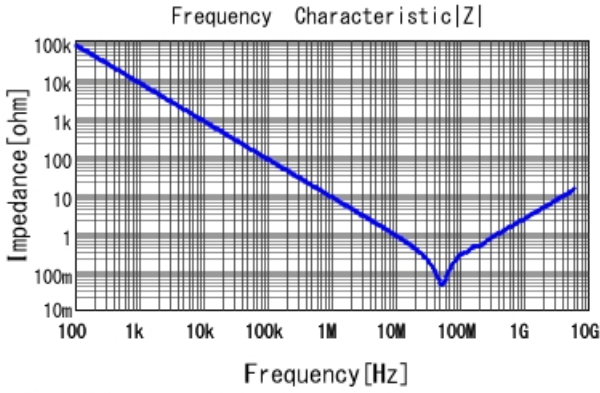
■ GCJ188R92A223KA01 |Z| DC0V, 25degC
