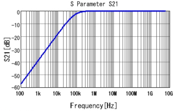
■ GCJ188R92A223KA01 S21 DCOV, 25degC
