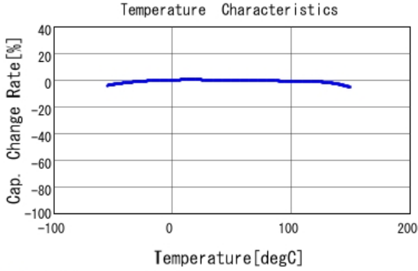
■ GCJ188R92A223KA01 C-Temp. capchange, DCO. 0V, AC1. 0Vrm
