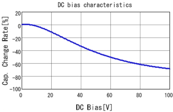
■ GCJ188R92A223KA01 C-DC bias capchange, 25.0degC, AC1.
