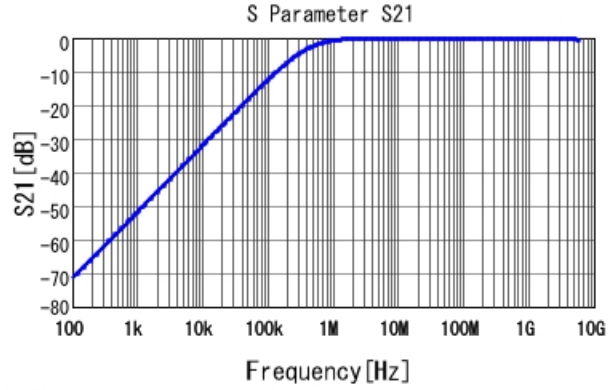
■ GCJ188R92A392KA01 S21 DCOV, 25degC
