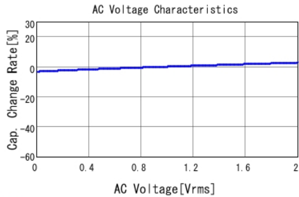
■ GCJ21BL81E224KA01 C-AC Voltage capchange, DC0V, 25.0d
