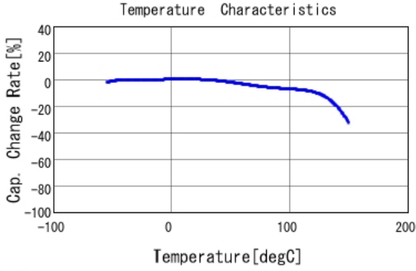
■ GCJ21BL8YA334KA01 C-Temp. capchange, DCO. 0V, AC1. 0Vrm
