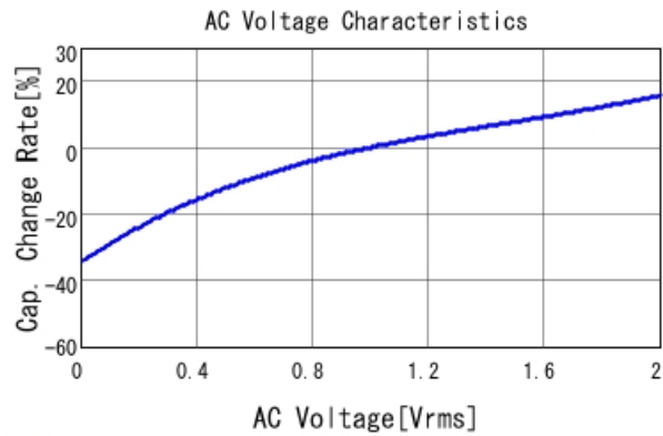
■ GCJ21BR71E225KA01 C-AC Voltage capchange, DC0V, 25.0d
