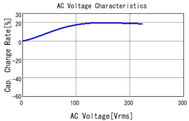
■ GCJ31BR72J152KXJ1 C-AC Voltage capchange, DC0V, 25.0d
