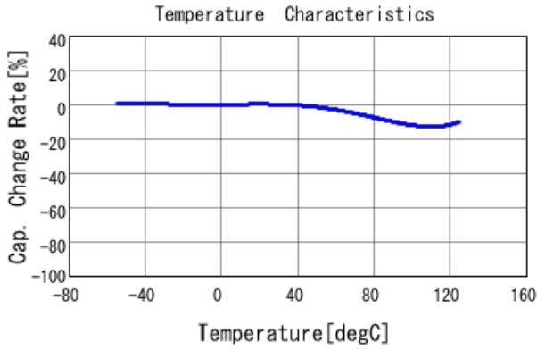
■ GCJ31BR72J152KXJ1 C-Temp. capchange, DCOV, AC1Vrms
