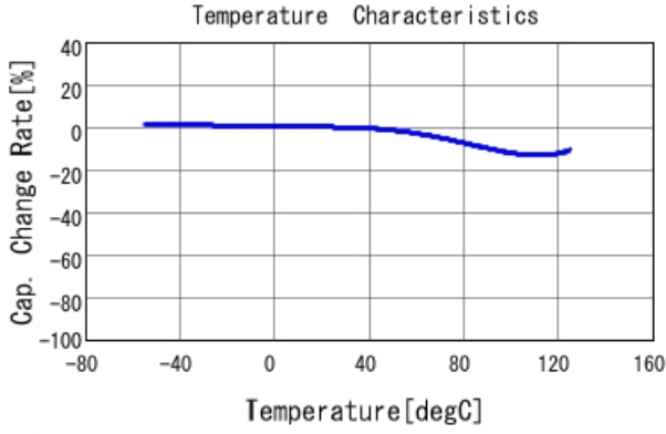
■ GCJ31BR72J332KXJ1 C-Temp. capchange, DCOV, AC1Vrms
