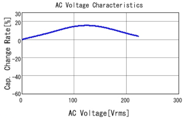
■ GCJ31BR72J332KXJ1 C-AC Voltage capchange, DC0V, 25.0d
