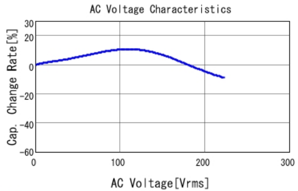
■ GCJ31BR72J682KXJ1 C-AC Voltage capchange, DC0V, 25.0d
