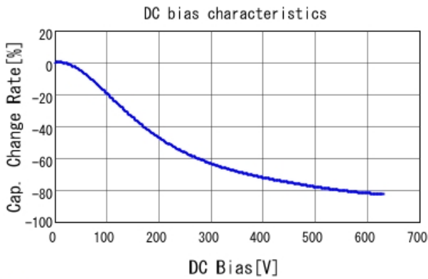
■ GCJ31BR72J682KXJ1 C-DC bias capchange, 25.0degC, AC1V
