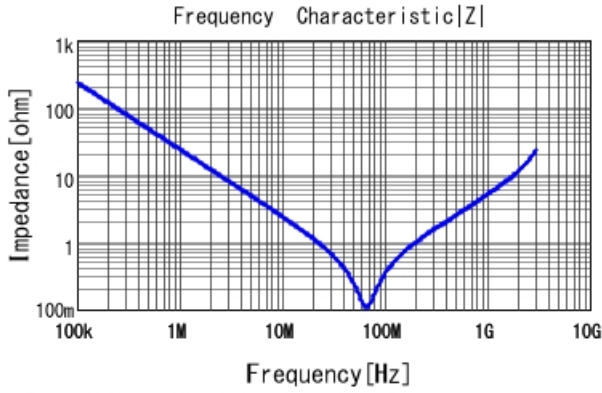
■ GCJ31BR72J682KXJ1 |Z| DC0V, 25degC
