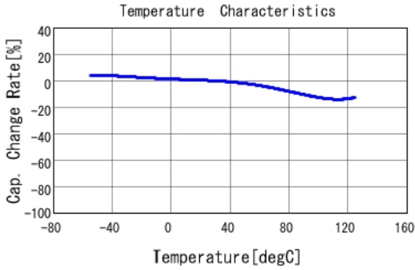
■ GCJ31BR72J682KXJ1 C-Temp. capchange, DCOV, AC1Vrms
