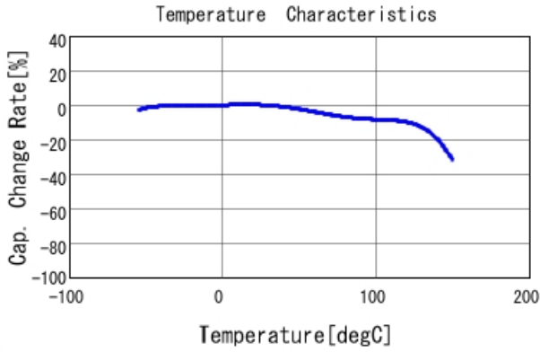
■ GCJ31CL8YA105KA01 C-Temp. capchange, DCO. 0V, AC1. 0Vrm
