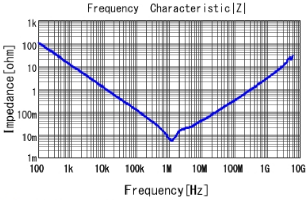
■ GCJ31CR70J226KE01 |Z| DC0V, 25degC
