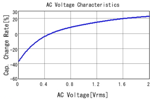
■ GCJ31CR70J226KE01 C-AC Voltage capchange, DC0V, 25.0d
