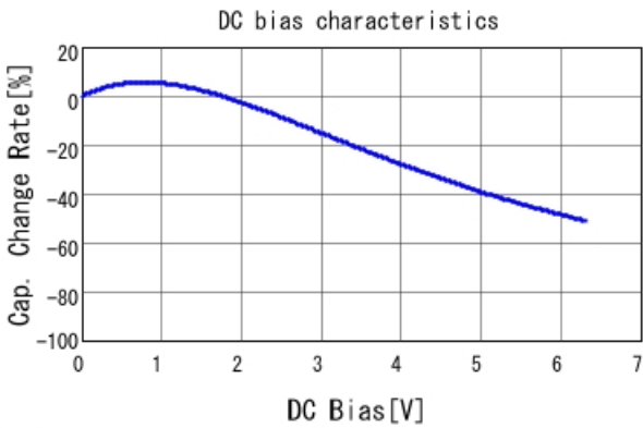
■ GCJ31CR70J226KE01 C-DC bias capchange, 25.0degC, AC0.
