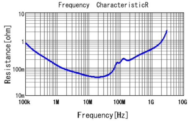
■ GCJ31CR72J223KXJ3 R DC0V, 25degC
