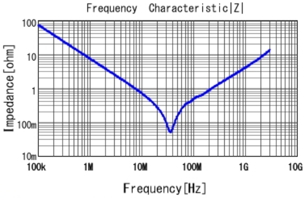
■ GCJ31CR72J223KXJ3 |Z| DC0V, 25degC
