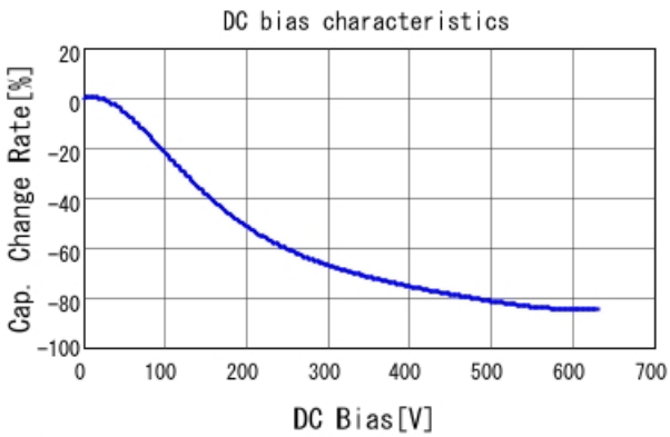
■ GCJ31CR72J223KXJ3 C-DC bias capchange, 25.0degC, AC1V
