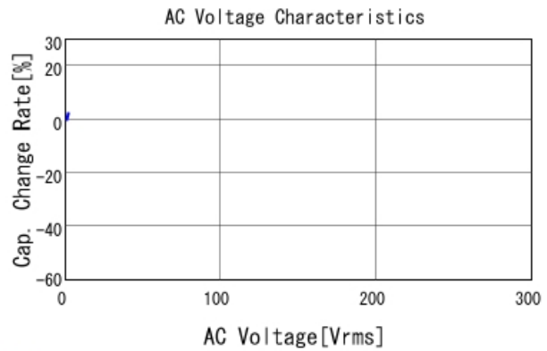
■ GCJ31CR72J223KXJ3 C-AC Voltage capchange, DC0V, 25.0d
