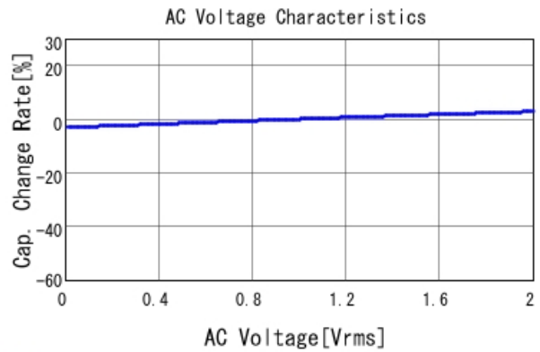
■ GCJ31MR71H474KA01 C-AC Voltage capchange, DCOV, 25.0d
