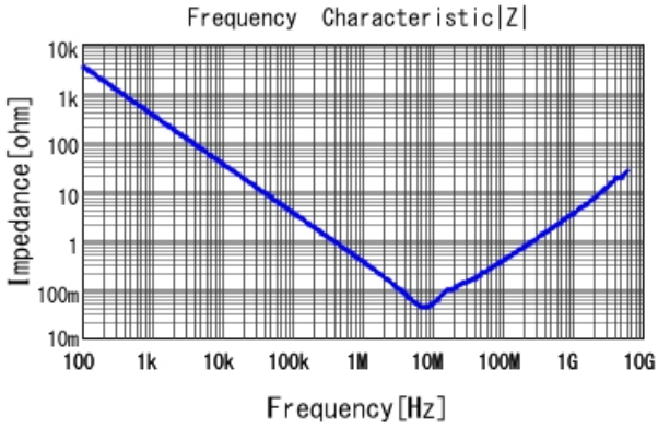
■ GCJ31MR71H474KA01 |Z| DCOV, 25degC
