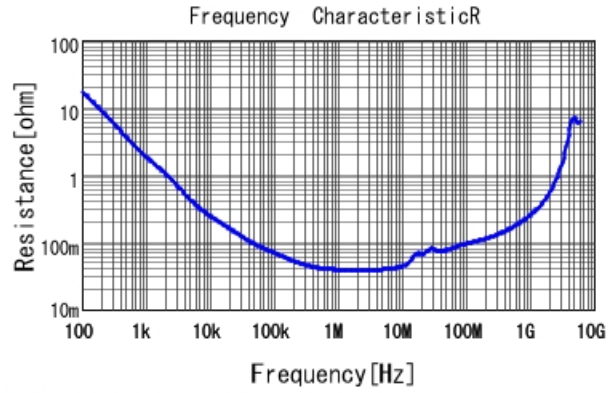
■ GCJ31MR71H474KA01 R DCOV, 25degC
