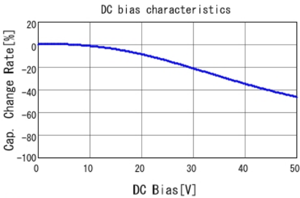
■ GCJ31MR71H474KA01 C-DC bias capchange, 25.0degC, AC1.
