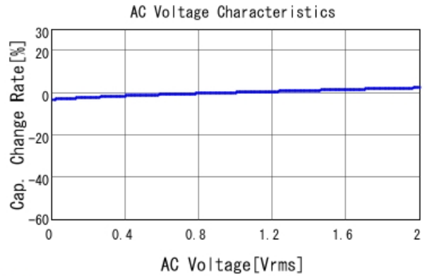
■ GCJ31MR72A184KA01 C-AC Voltage capchange, DCOV, 25.0d
