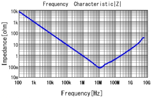
■ GCJ31MR72A224KA01 |Z| DCOV, 25degC
