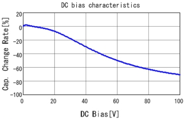
■ GCJ31MR72A224KA01 C-DC bias capchange, 25.0degC, AC1.
