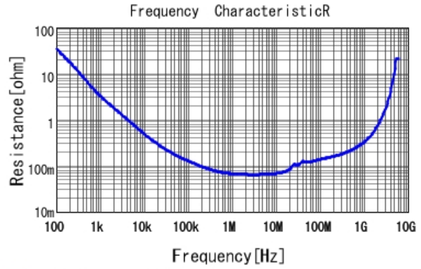
■ GCJ31MR72A224KA01 R DCOV, 25degC
