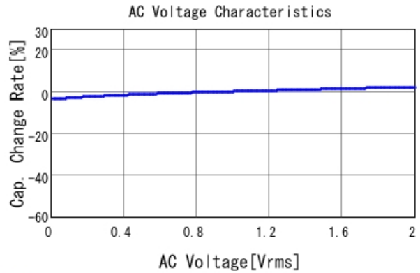
■ GCJ31MR72A224KA01 C-AC Voltage capchange, DCOV, 25.0d
