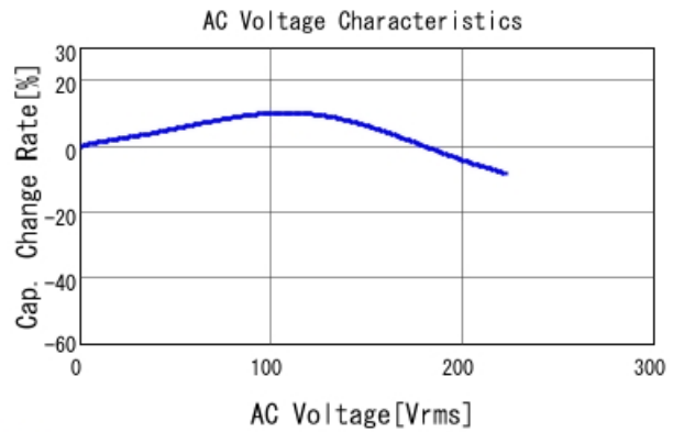
■ GCJ32DR72J333KXJ1 C-AC Voltage capchange, DC0V, 25.0d
