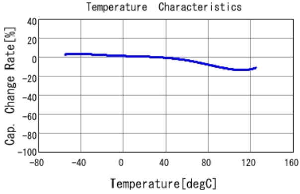
■ GCJ32DR72J333KXJ1 C-Temp. capchange, DCOV, AC1Vrms
