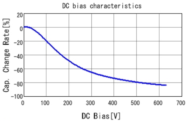
■ GCJ32DR72J333KXJ1 C-DC bias capchange, 25.0degC, AC1V
