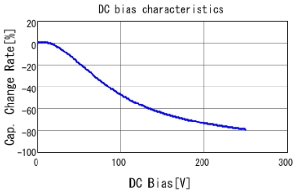
■ GCJ43DR72E474KXJ1 C-DC bias capchange, 25.0degC, AC1V
