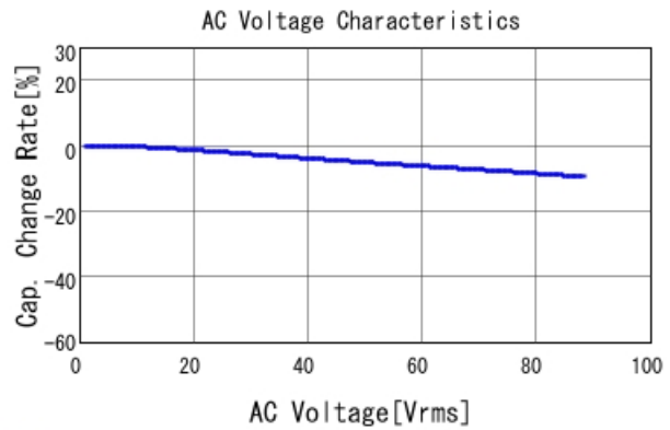
■ GCJ43DR72E474KXJ1 C-AC Voltage capchange, DC0V, 25.0d
