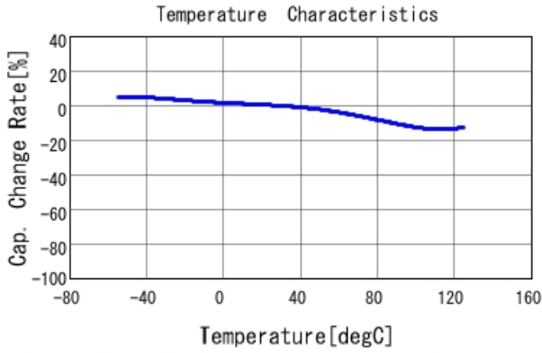
■ GCJ43DR72E474KXJ1 C-Temp. capchange, DCOV, AC1Vrms
