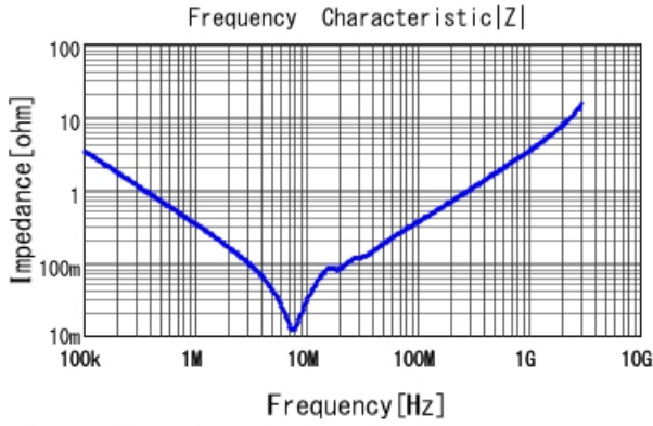
■ GCJ43DR72E474KXJ1 |Z| DC0V, 25degC
