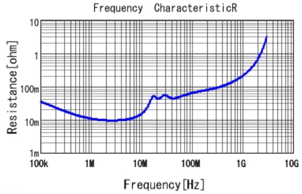
■ GCJ43DR72E474KXJ1 R DC0V, 25degC
