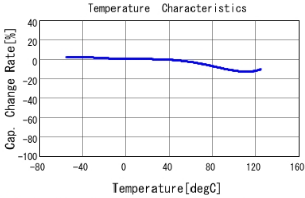
■ GCJ43DR72J333KXJ1 C-Temp. capchange, DCOV, AC1Vrms
