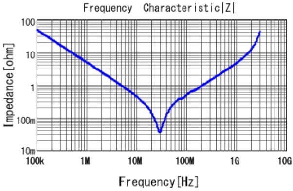
■ GCJ43DR72J333KXJ1 |Z| DC0V, 25degC
