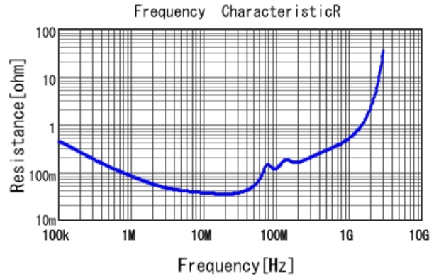
■ GCJ43DR72J333KXJ1 R DC0V, 25degC
