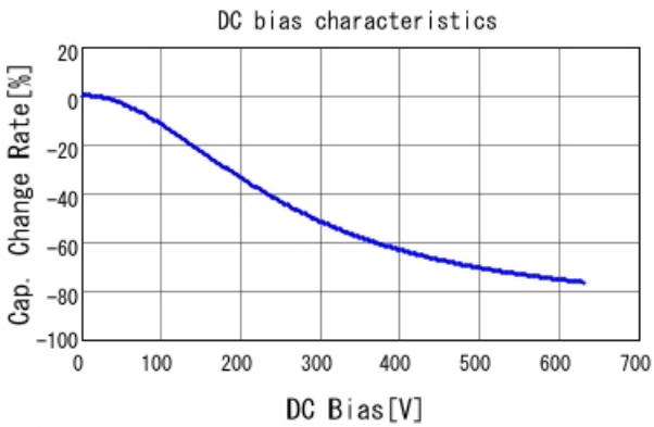
■ GCJ43DR72J333KXJ1 C-DC bias capchange, 25.0degC, AC1V
