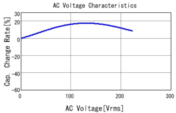
■ GCJ43DR72J333KXJ1 C-AC Voltage capchange, DC0V, 25.0d
