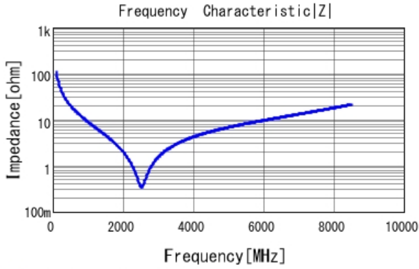
GCM0335C1E150FA16 |Z| DC0V, 25degC
