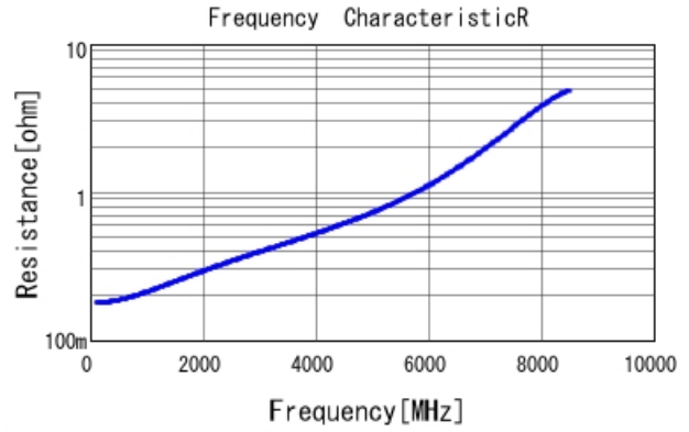
GCM0335C1E150FA16 R DC0V, 25degC
