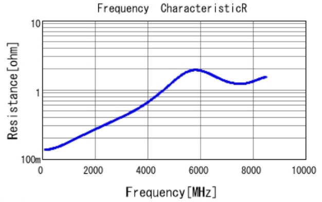
■ GCM0335C1E430FA16 R DC0V, 25degC
