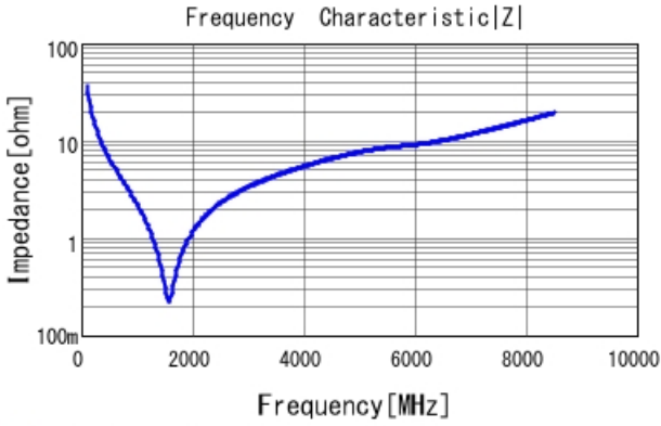
■ GCM0335C1E430FA16 |Z| DC0V, 25degC
