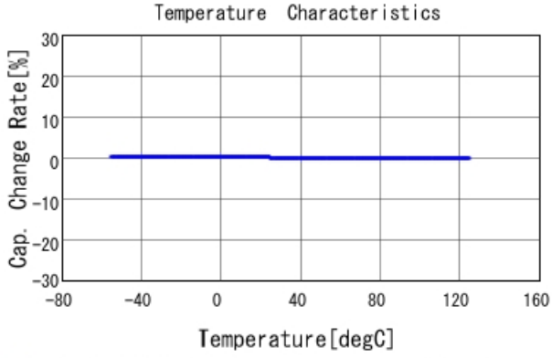
■ GCM0335C1H100FA16 C-Temp. capchange, DCOV, AC1Vrms
