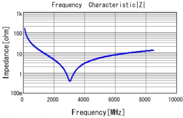
■ GCM0335C1H100FA16 |Z| DC0V, 25degC
