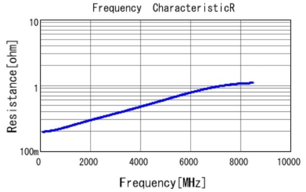
■ GCM0335C1H100FA16 R DC0V, 25degC
