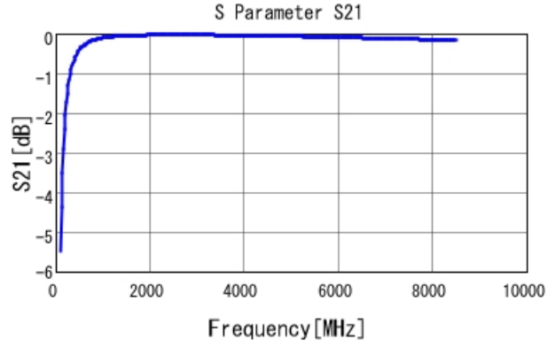
■ GCM0335C1H100FA16 S21 DCOV, 25degC
