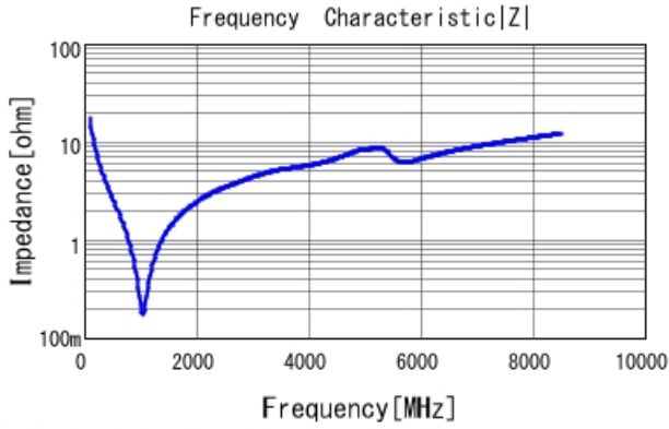
GCM0335C1H910FA16 |Z| DCOV, 25degC
