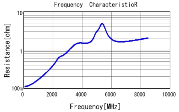
GCM0335C1H910FA16 R DCOV, 25degC
