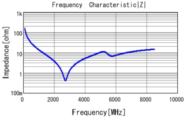
GCM1555C1H100GA16 |Z| DC0V, 25degC
