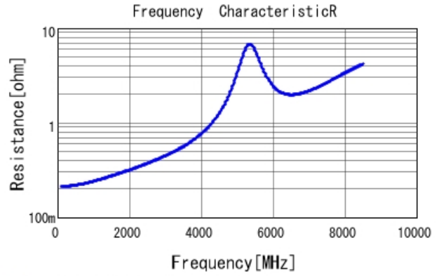
GCM1555C1H100GA16 R DC0V, 25degC
