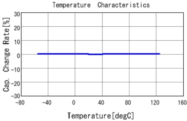
■ GCM1555C1H1R0BA16 C-Temp. capchange, DCOV, AC1Vrms
