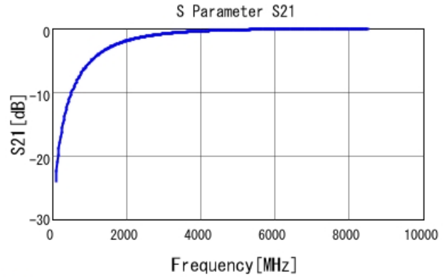
■ GCM1555C1H1R0BA16 S21 DCOV, 25degC
