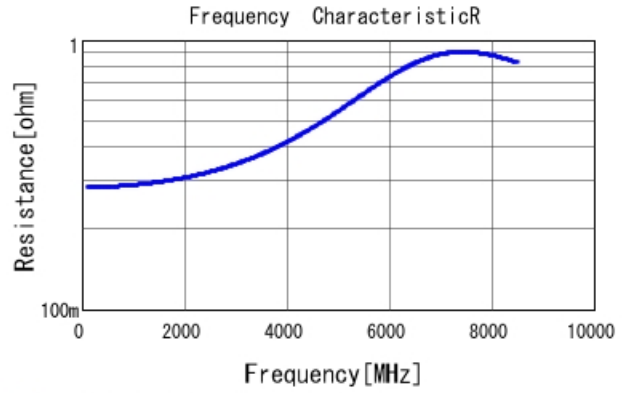
GCM1555C1H2R7WA16 R DCOV, 25degC
