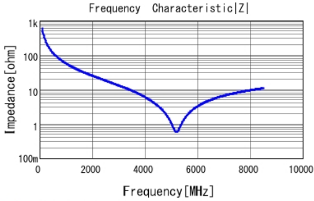
GCM1555C1H2R7WA16 |Z| DCOV, 25degC
