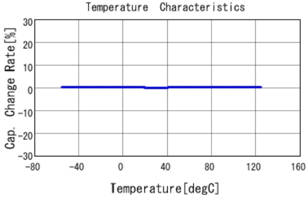
■ GCM1555C1H4R7BA16 C-Temp. capchange, DCOV, AC1Vrms
