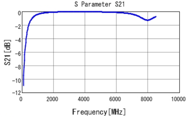
■ GCM1555C1H4R7BA16 S21 DCOV, 25degC
