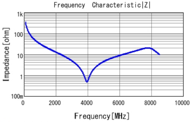
■ GCM1555C1H4R7BA16 |Z| DC0V, 25degC
